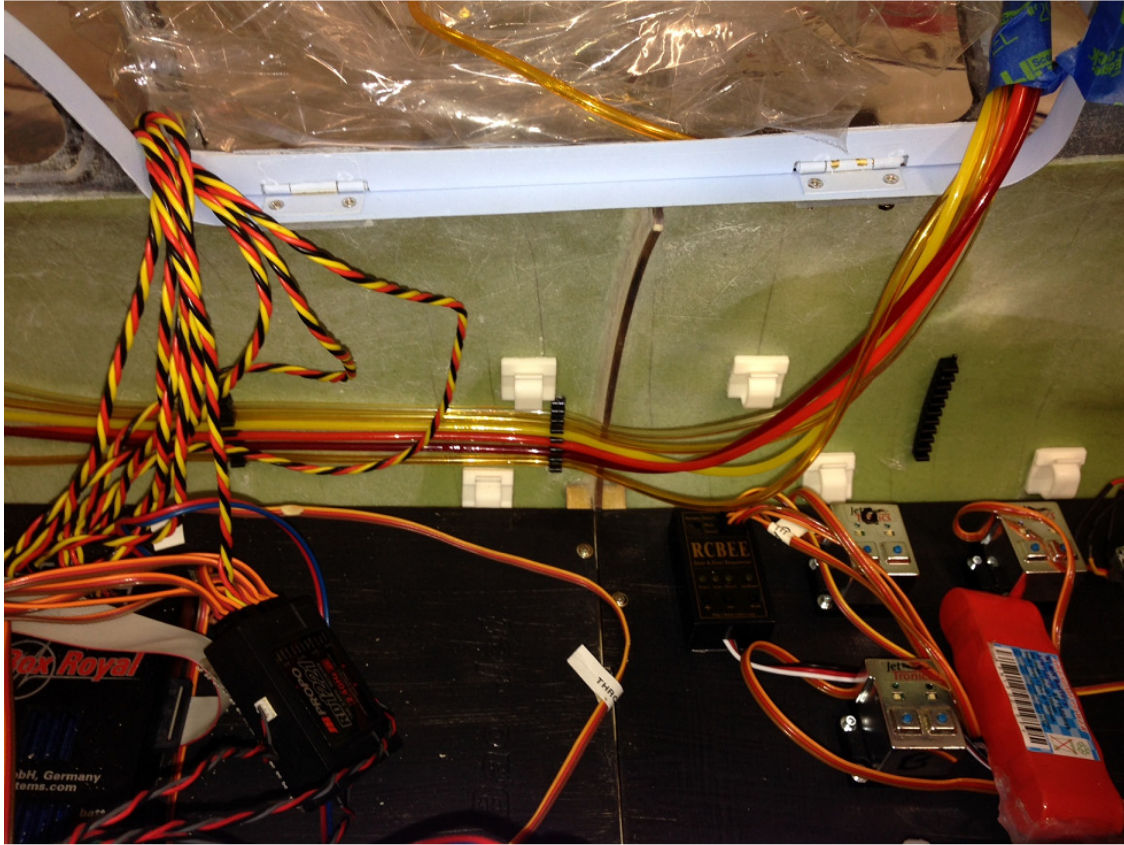
Photo 4 – air lines colour coded and run to the centre area of the component boards. The Speed brake air lines have been run to this spot too.
