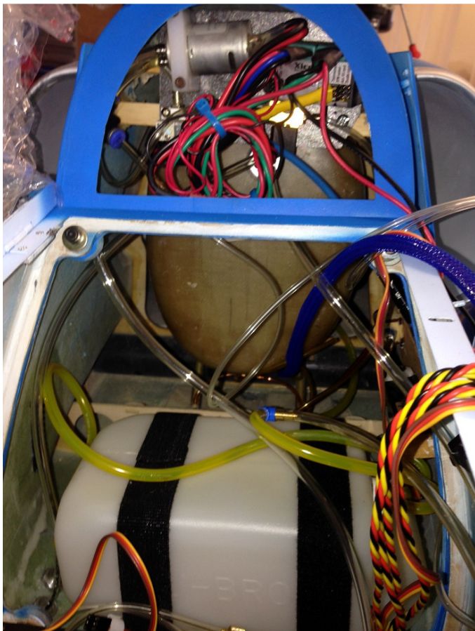
Photo 2 – Smoke Tank Layout added for Deisel. I used a normal Dubro tank for the smoke tank. (everything has not been secured yet so it looks messy)
