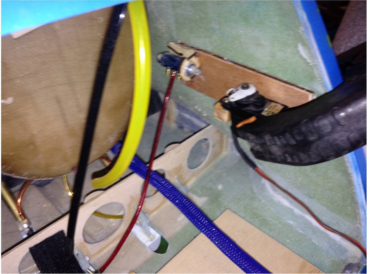
Photo 6 – view of the speed brakes and servo and valve mounted on the site of fuse.
