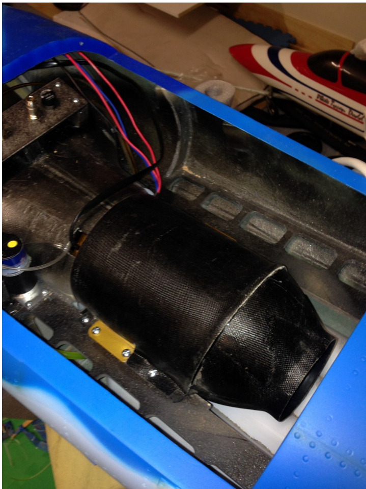
Photo 7&8 – mounting thrust tube, bypass and engine.
